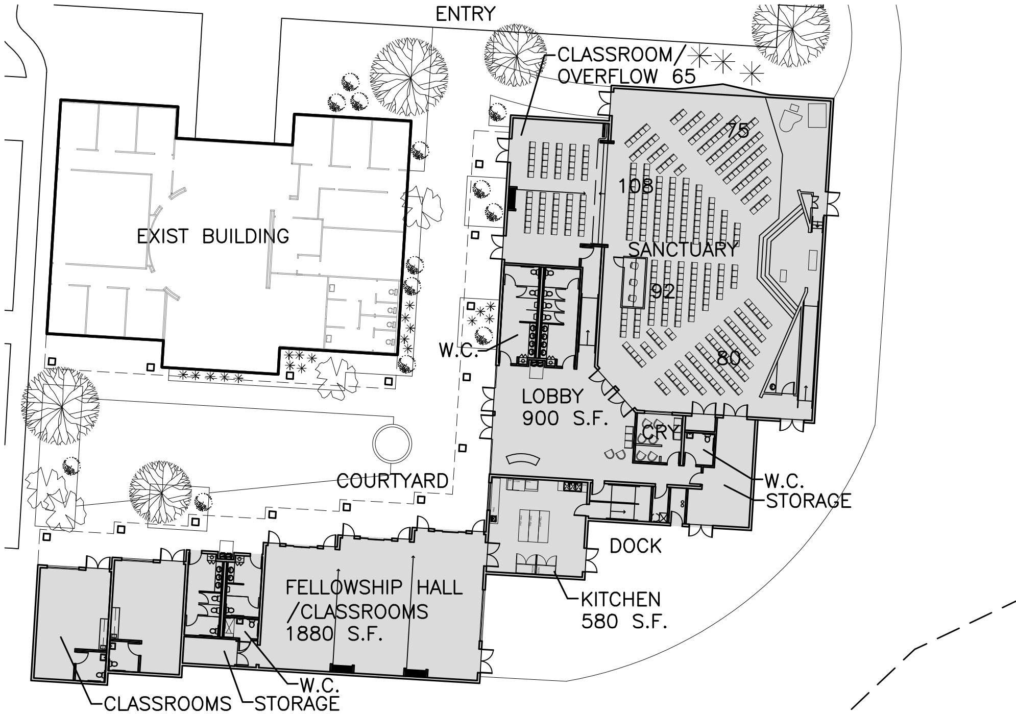
CONCEPT PLAN 'G' N.T.S. 4.28.16 TOTAL SF = 12,419 S.F.
